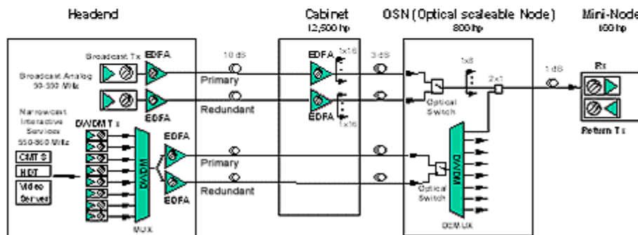
Figure 2: DWDM Deep Fiber HFC Architecture - Forward Path
