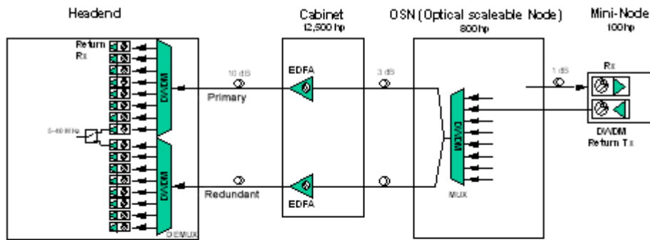
Figure 4: Deep Fiber HFC Architecture - Pure DWDM Return Path
