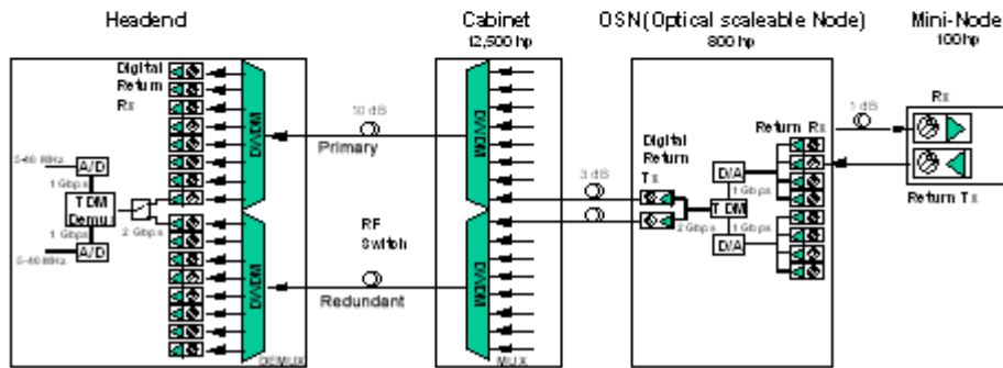
Figure 5: Deep Fiber HFC Architecture - Digital/DWDM Return Path
