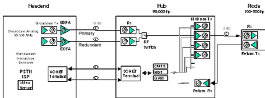
Figure 1: Traditional HFC Architecture
